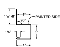
14 National Track Cover 10'-6" 42808
