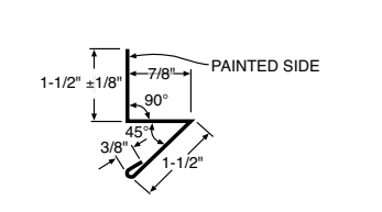
15 Cannonball Track Cover 10'-6" 42700
