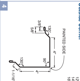
Outside Corner 10-6" 42183 10-6" 42185 14-6" 42186 16-6" 42187
