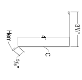
1 Image II Rake 10-2° 55951 / 58951
