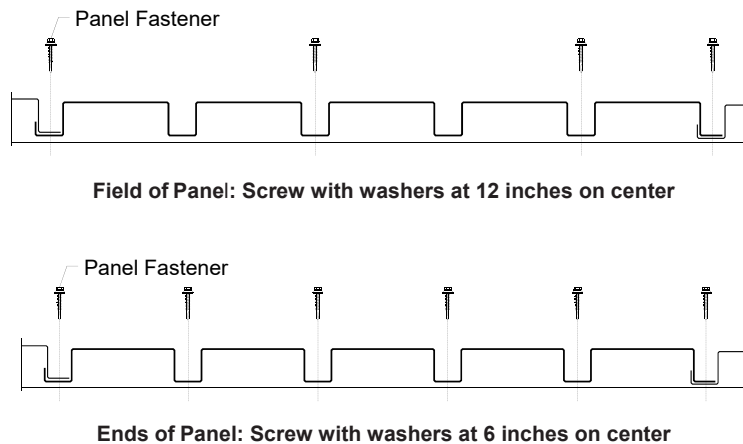
FIGURE 4—T10-C PANEL PROFILE AND FASTENING SCHEDULE FOR T10-C WALL PANELS
