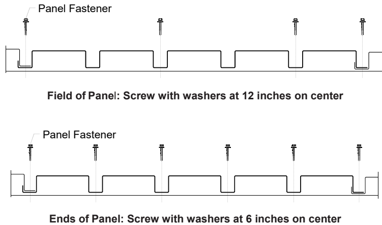
FIGURE 4—T10-C PANEL PROFILE AND FASTENING SCHEDULE FOR T10-C WALL PANELS
