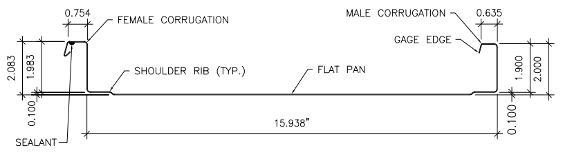
PANEL SECTION (MIN 0.032" THICK ALUMINUM)
