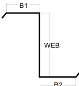
(Symmetrical Flange)
