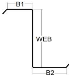
(Unsymmetrical Flange)
