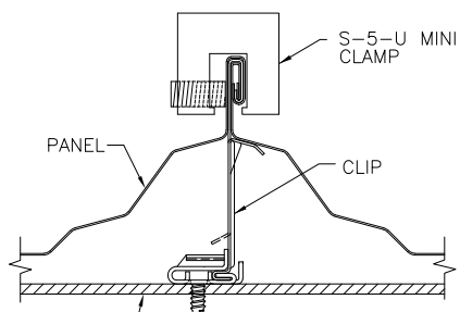
CLIP SECTION VIEW
