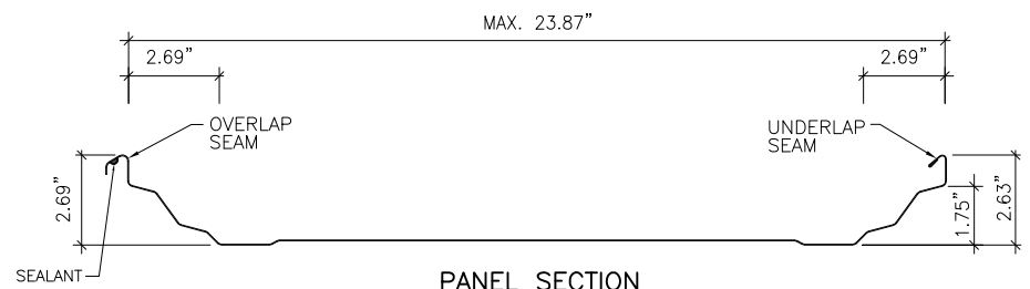
PANEL SECTION (MIN 24 GA.)
