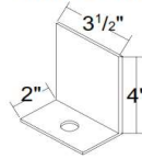
ANGLE CLIP
