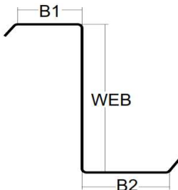
(Unsymmetrical Flange)
