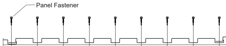
Ends of Panel: Screw with washers at 9 inches on center
