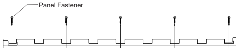
Field of Panel: Screw with washers at 4.5 inches on center
