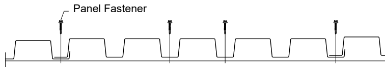
Field of Panel: Screw with washers at 12 inches on center
