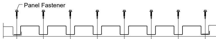
Ends of Panel: Screw with washers at 4 inches on center
