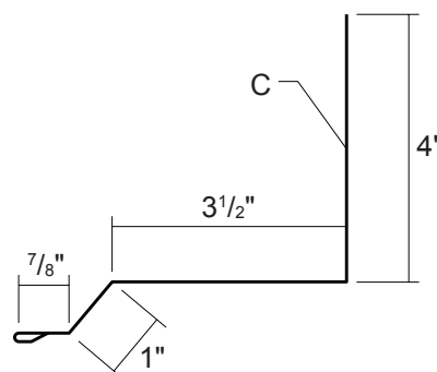
5► UNIVERSAL SIDEWALL
