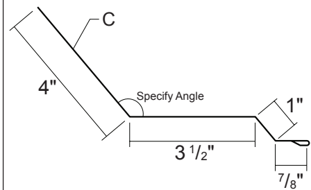
6► VALLEY
