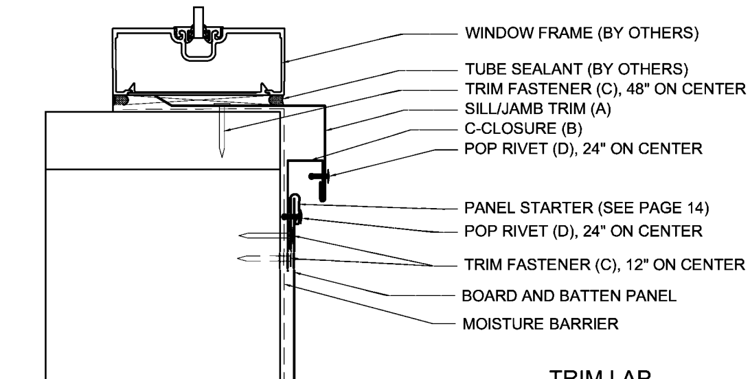
ELEVATION VIEW
