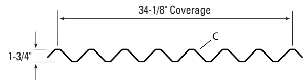
T12 Wall
