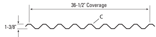
T16-E Wall
