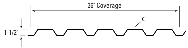
T7 Wall
